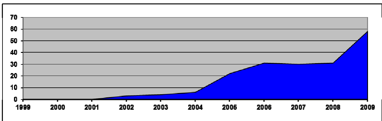
Chart 1-c - The number of identified domestic victims
