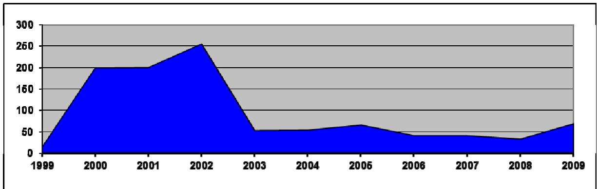
Chart 1-b - The number of identified foreign victims.
